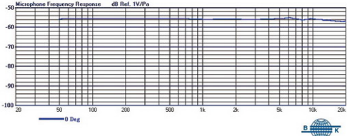
Frequency Response
